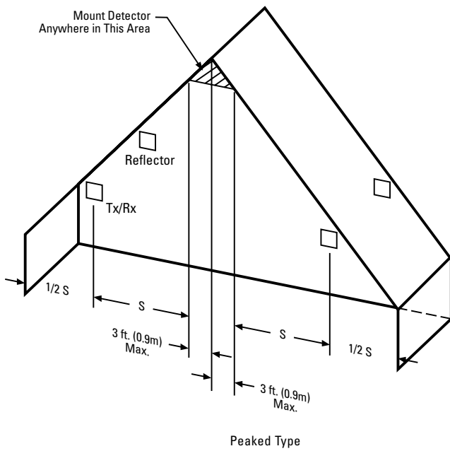
Figures 10 and 11. Mounting on Sloped Ceilings
