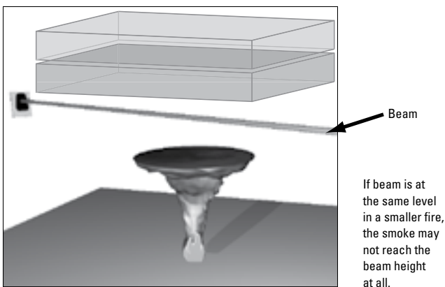
Figures 5, 6, 7. Pre-stratification and detector placement
