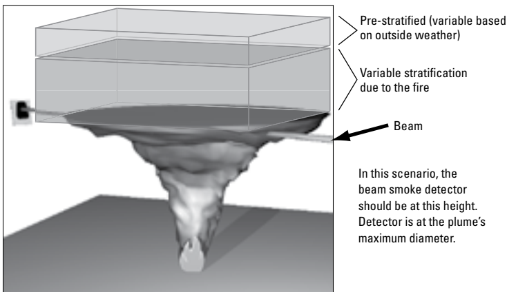
Figure 4. Typical smoke field in the shape of an inverted cone
